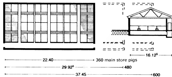
⑤ Store pig shed with rack stalls (120 animals per section)
